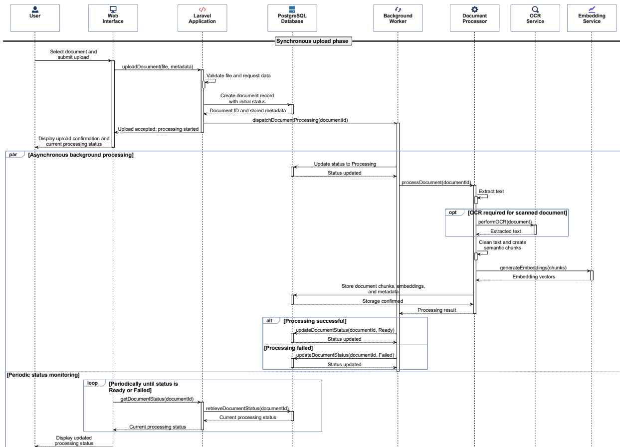
Figure 17: Sequence Diagram for Document Upload and Processing Workflow
