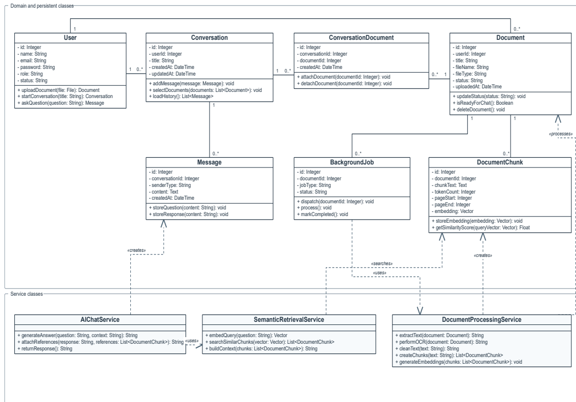
Figure 16: UML Class Diagram of the AI-Powered Enterprise RAG System
