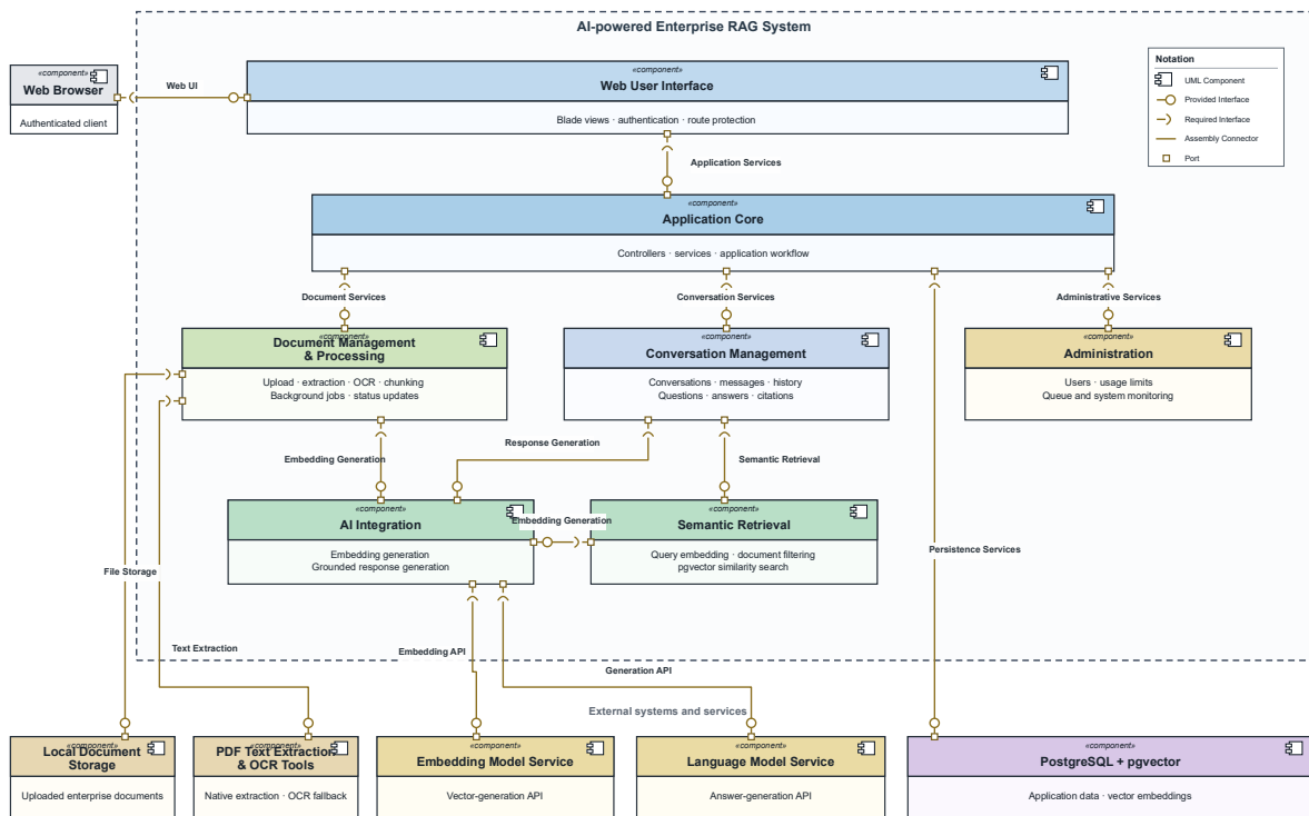
Figure 15: UML Component Diagram of the AI-Powered Enterprise RAG System
