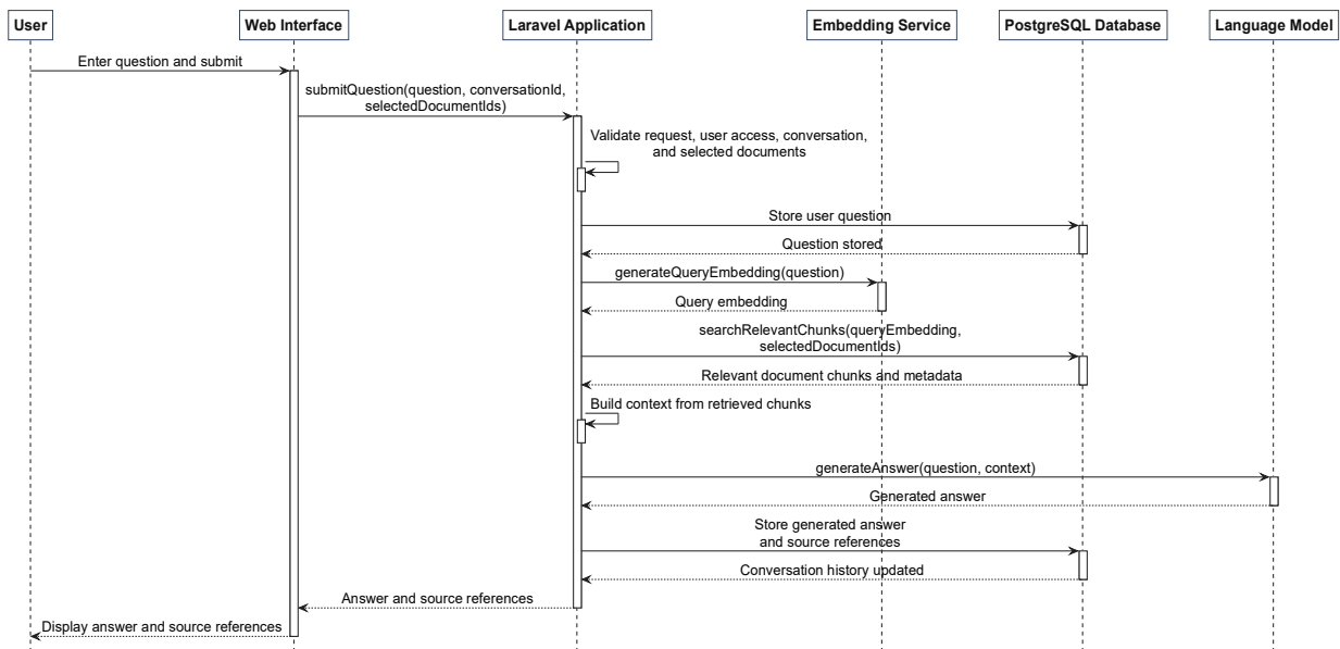
Figure 18: Sequence Diagram for AI-Assisted Question Answering Workflow
